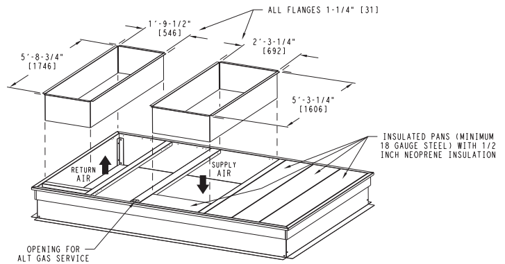
Fig. 5 - Roof Curb Details - Size 17 Unit
