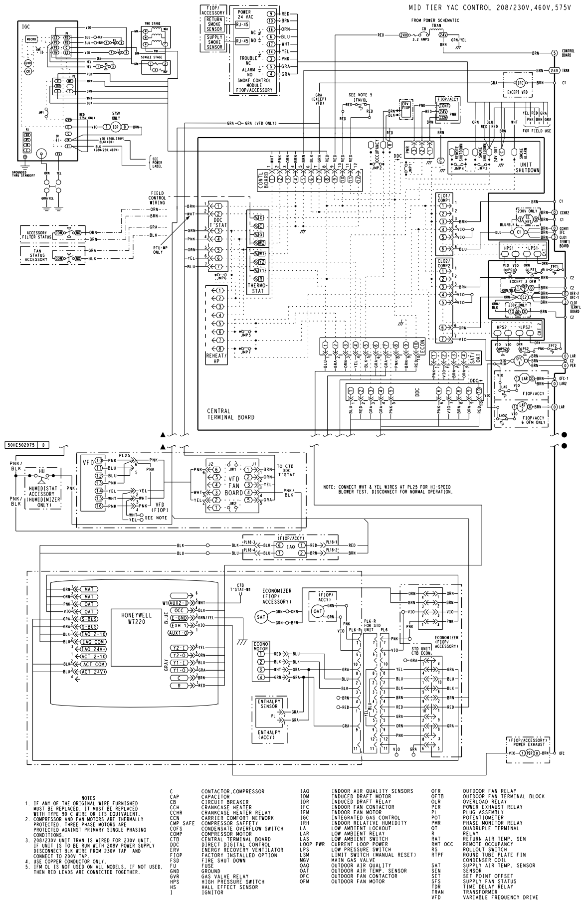
Fig. 19 - Electro-mechanical Control Wiring Diagram 48HC 17-24
