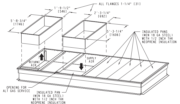
Fig. 15 - Roof Curb Details - Size 28 Unit
