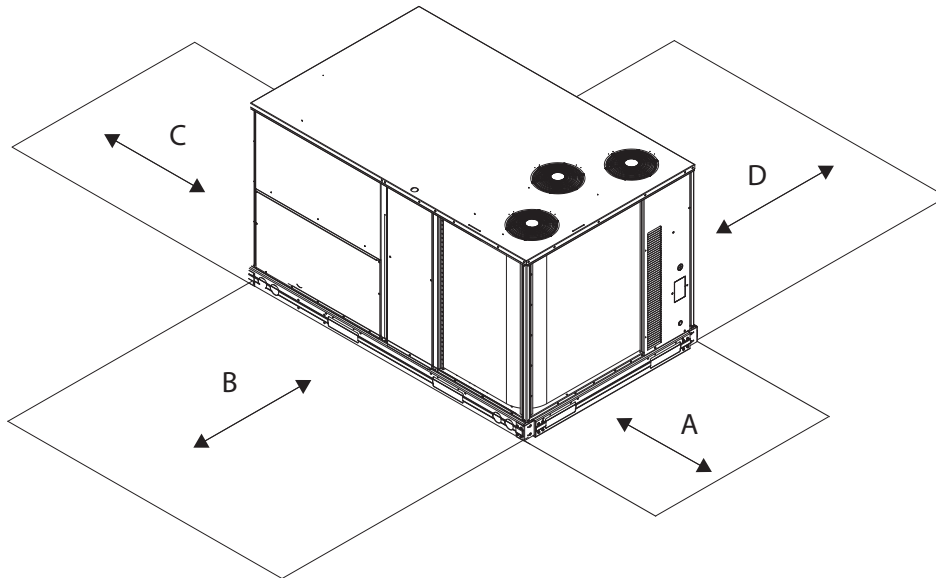
Fig. 4 - Service Clearance
