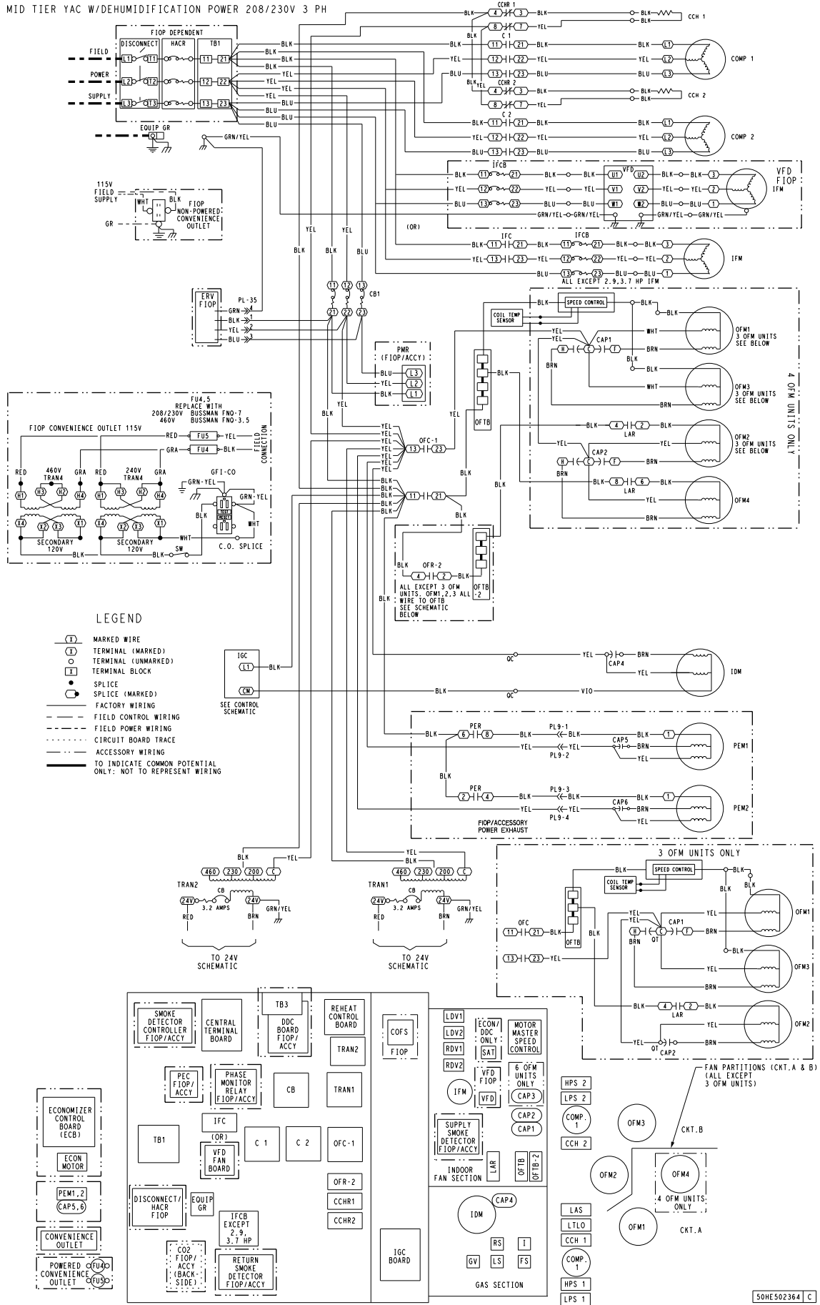
Fig. 22 - Typical Power Wiring Diagram for unit with Optional Humidi-MiZer® System, 48HC 17-24 208/230V shown
