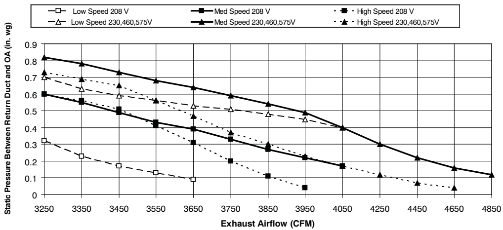
Fig. 18 - Power Exhaust Fan Performance
