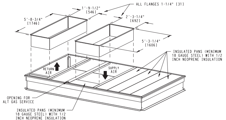
Fig. 10 - Roof Curb Details - Size 20 - 24 Units
