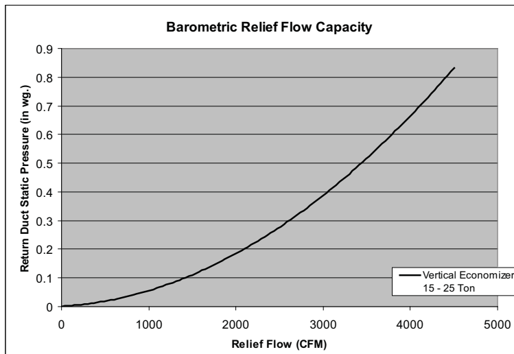
Fig. 17 - Barometric Relief Flow Capacity
