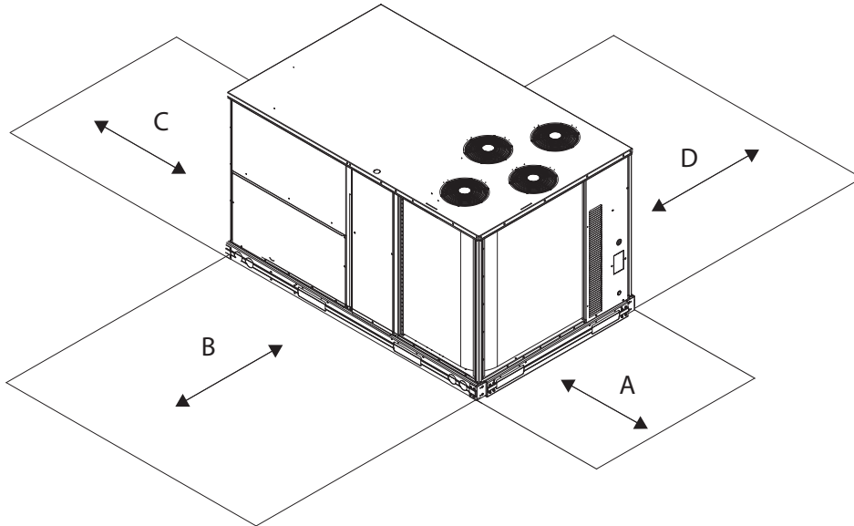
Fig. 9 - Service Clearance
