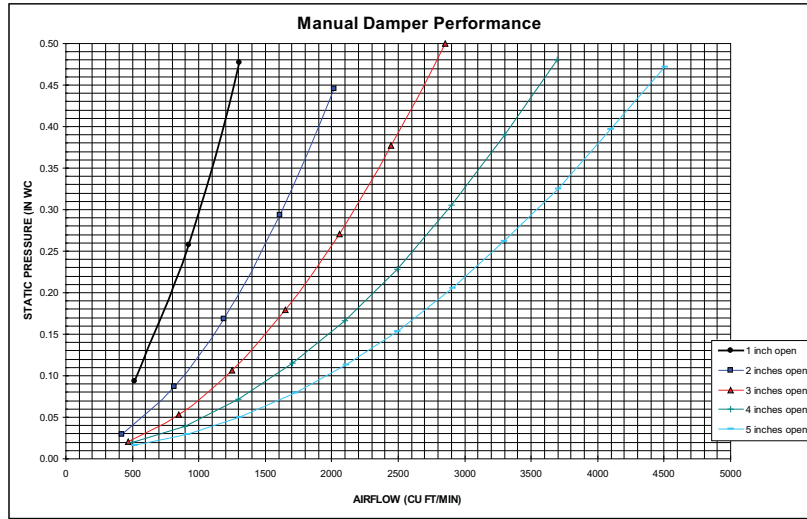
Fig. 16 - Manual Damper Performance
