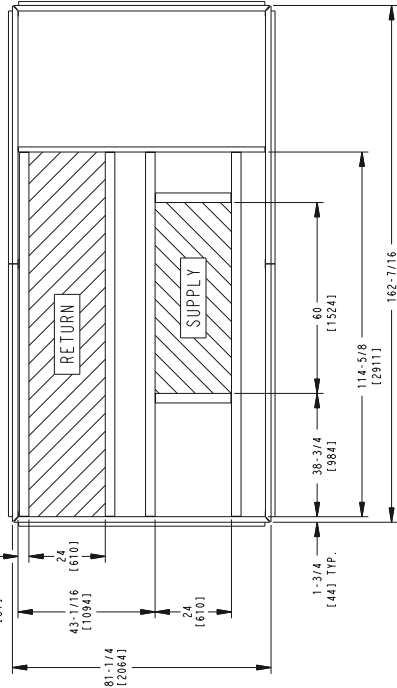
ROOF CURB DETAIL "A" (ALL OTHERS)
