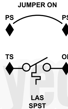
Fig. 24 - Schematic of SPST Low Ambient Switch
