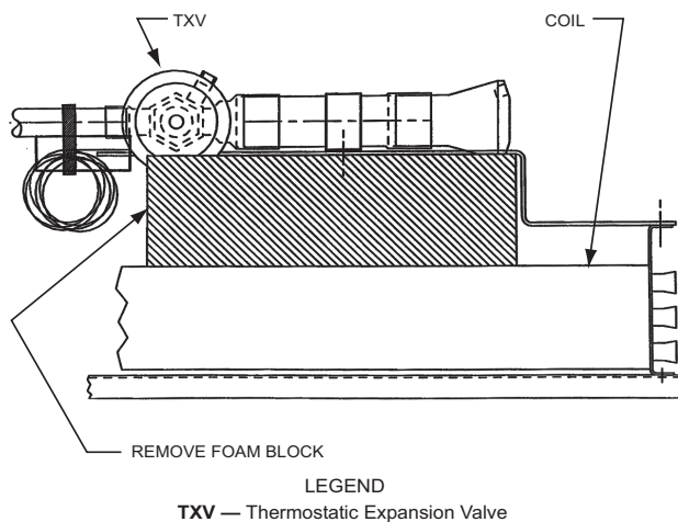
Fig. 5 - Foam Block Location
