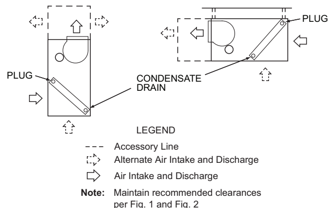
Fig. 6 - Typical Unit Positioning
