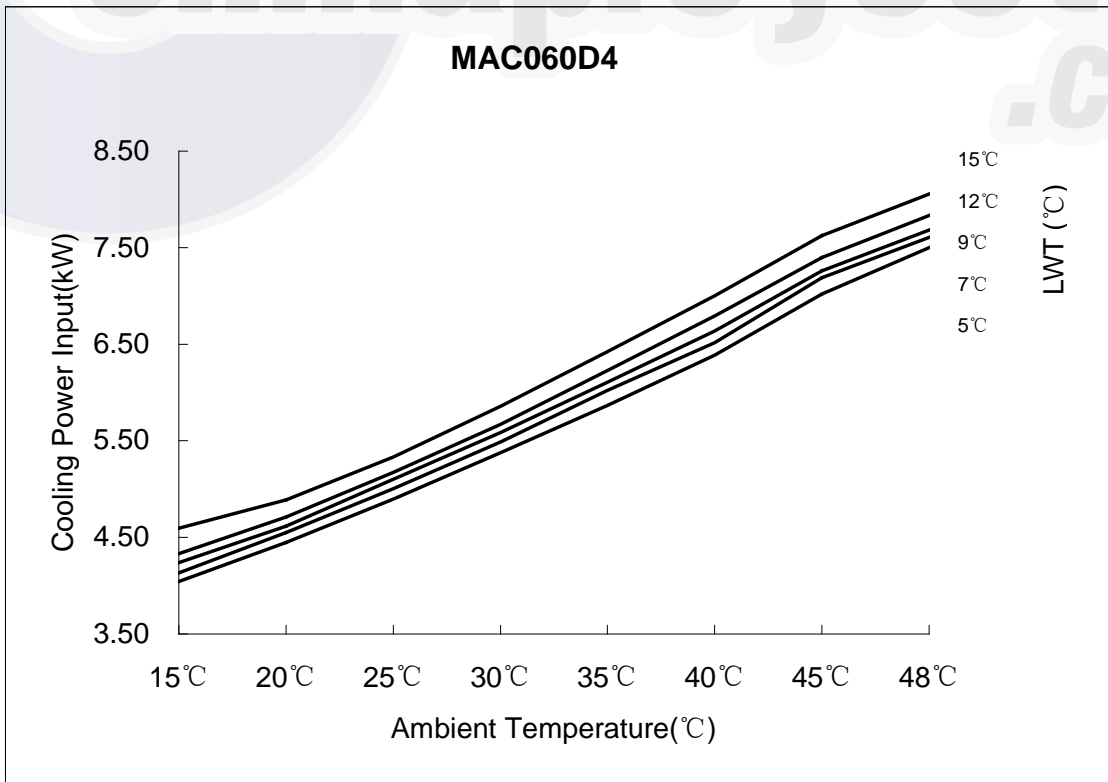
Cooling Power Input Char
