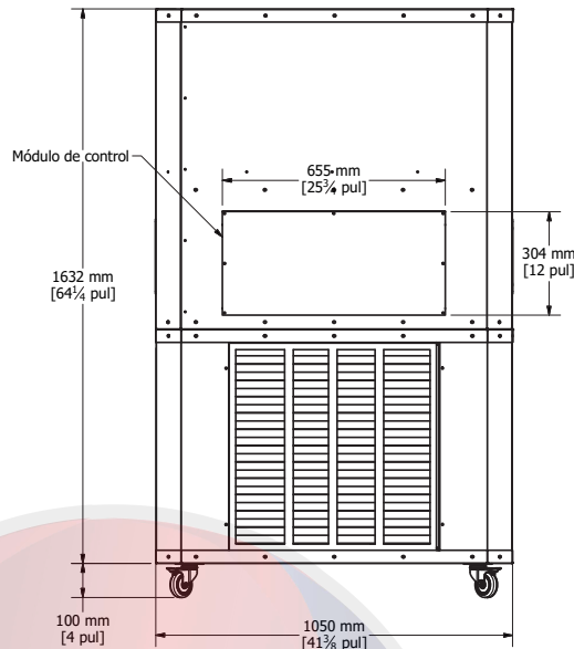
Vista Frontal
