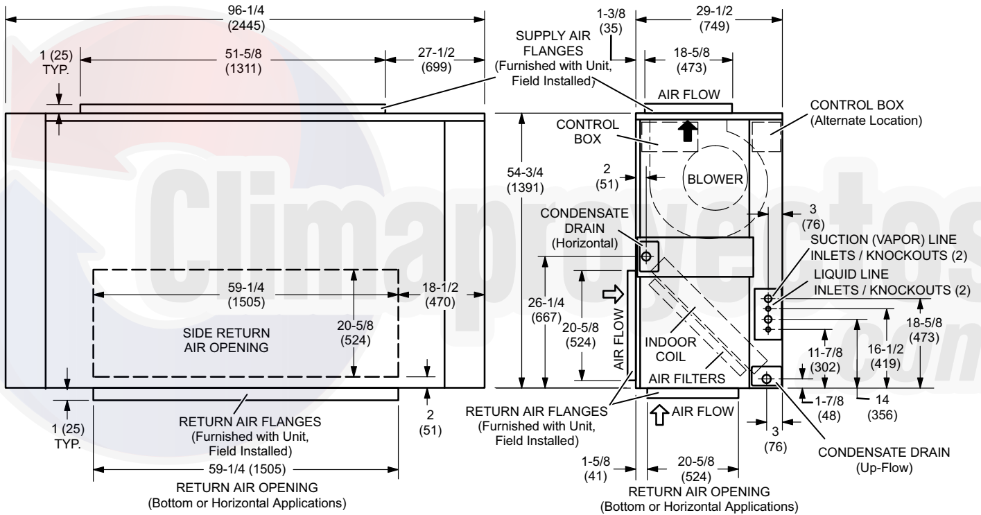
INLET VIEW
