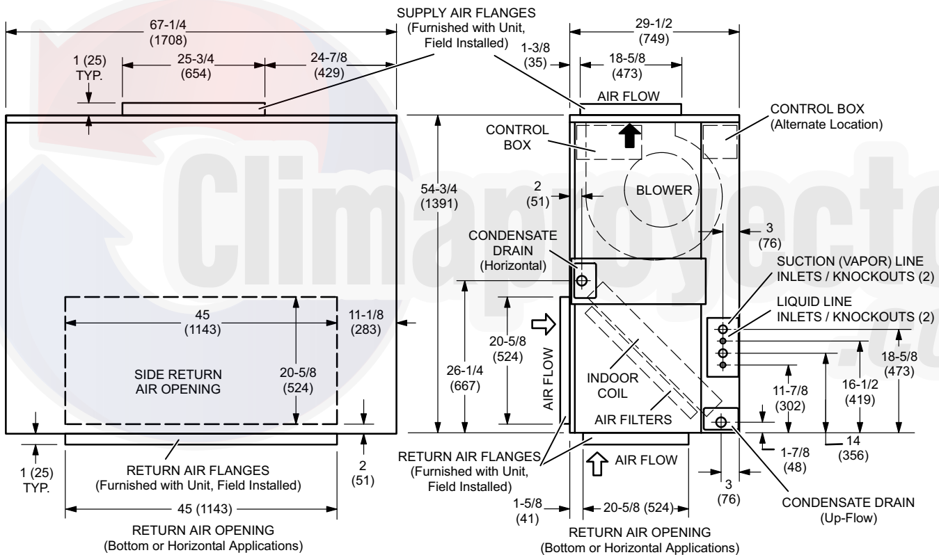
INLET VIEW
