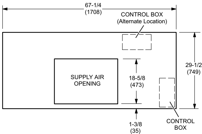
SUPPLY END VIEW
