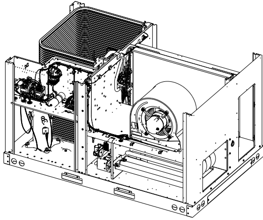
CONTROL BOX
