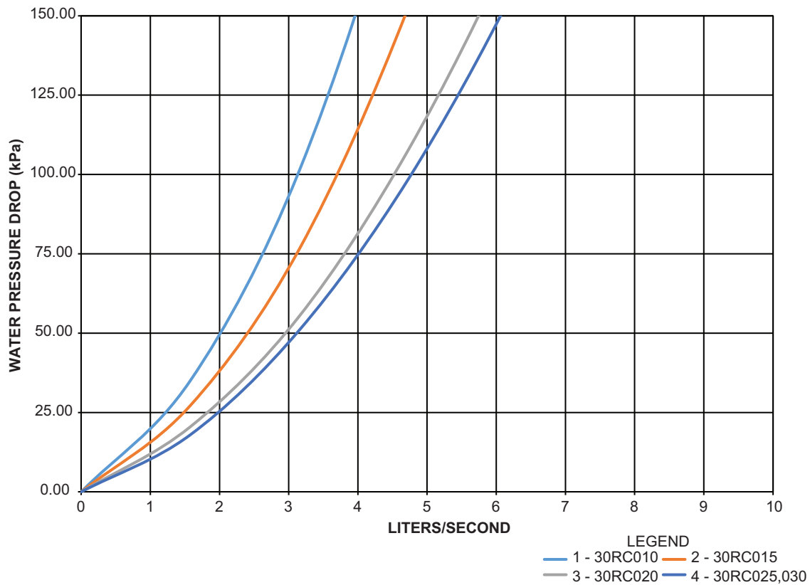
Unit Pressure Drop — Dual Pump Hydronic Package — 30RC010-030 (SI)
