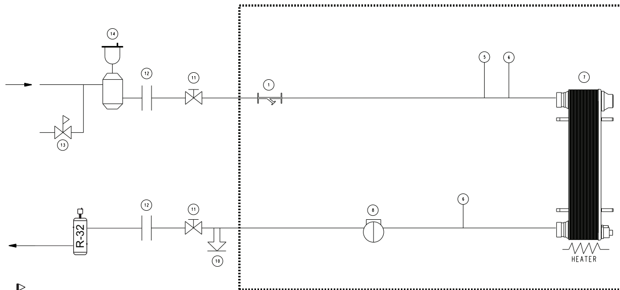
Typical Piping Diagram on 30RC Units Without Hydronic Package
