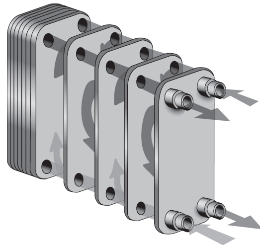
Brazen Plate Evaporator (Alternate Paths for Refrigerant and Water Flow)
