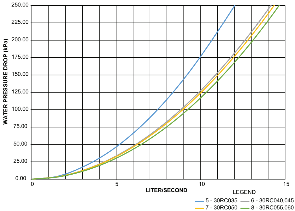
Unit Pressure Drop — Single Pump Hydronic Package — 30RC035-060 (SI)
