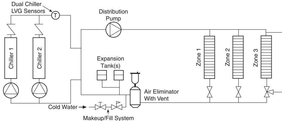
Typical Multiple Chiller Configuration with Air Eliminator and Expansion Tank Location
