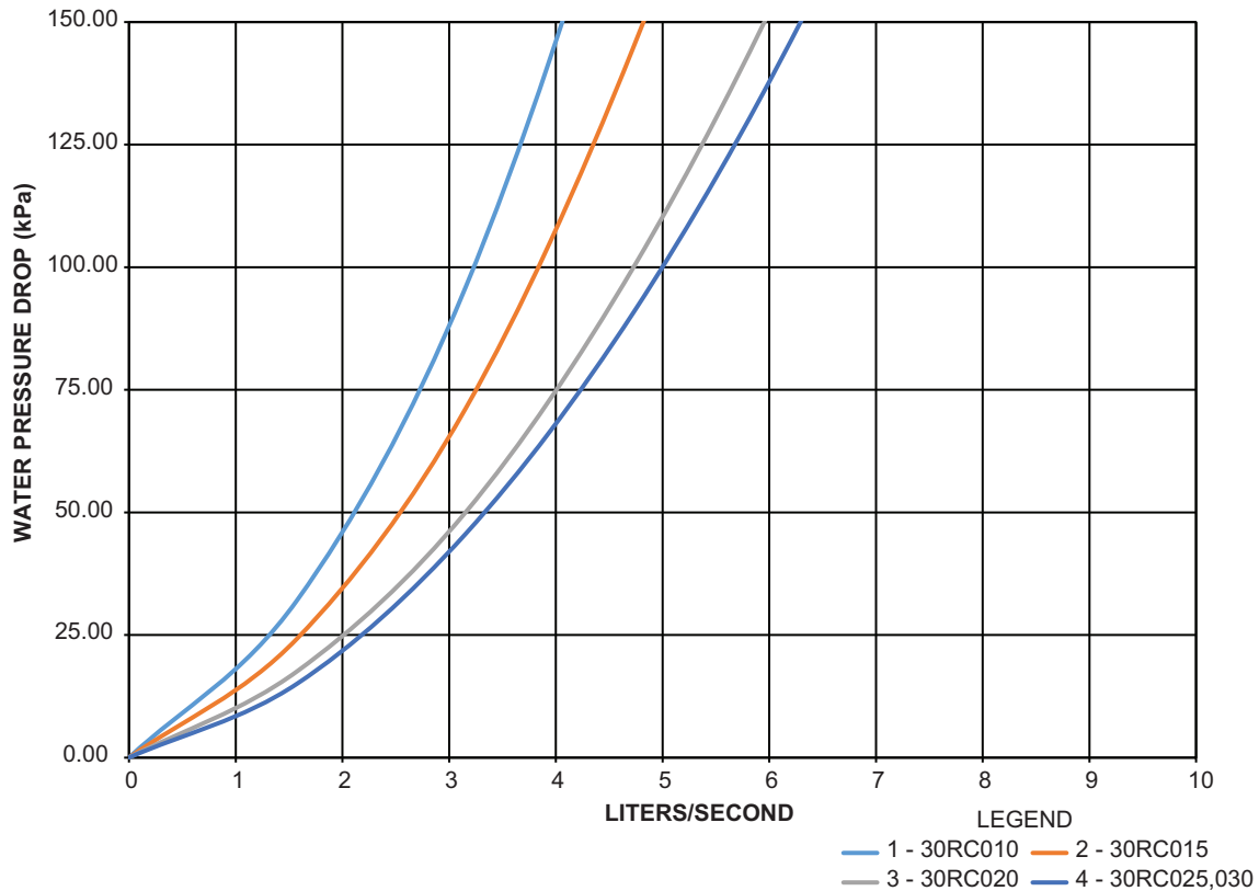
Unit Pressure Drop — Single Pump Hydronic Package — 30RC010-030 (SI)
