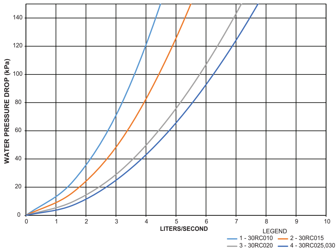
Heat Exchanger Pressure Drop — 30RC010-030 (SI)
